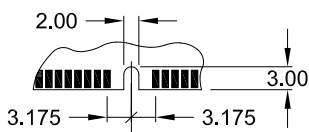
Module keying Type "A"
