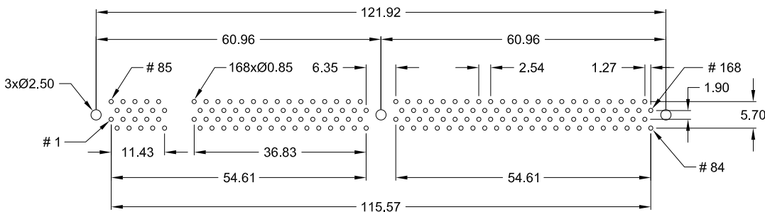
Module keying Type "A"
