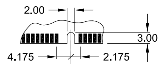
Module keying Type "C"
