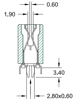
Metal Peg (Option)
