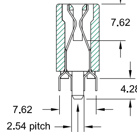
Plastic Peg (Standard)
