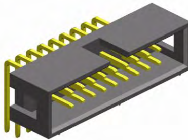
Right Angle Box Header
